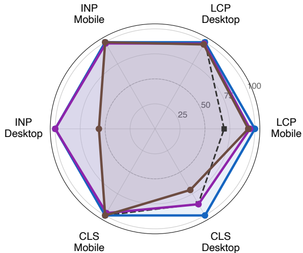
(a) Agent ablation (LLM = GPT-5)
