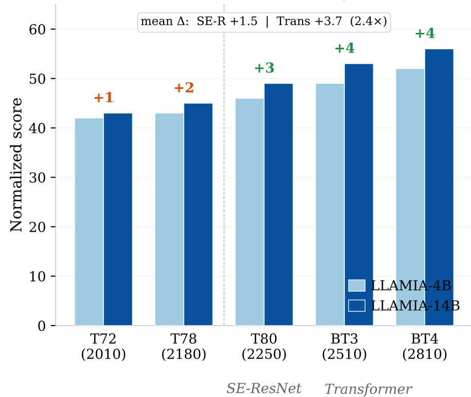
Behavior Cloning
