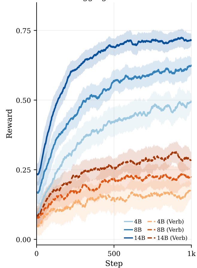
Aggregate reward
