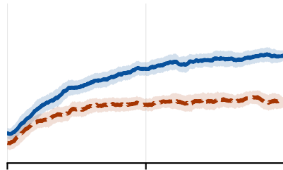
Difficulty
