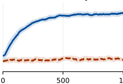
Game Commentary
