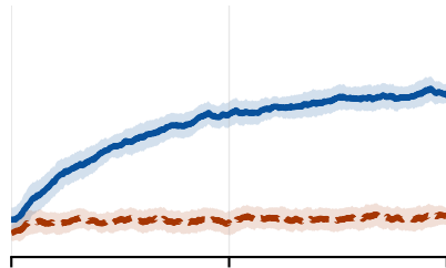
Interest
