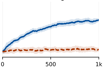
Instruction Planning
