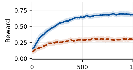
Rationale Prediction
