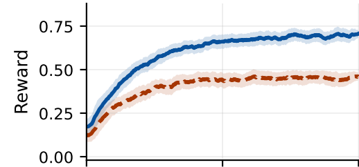
Behavior Cloning (MAIA)
