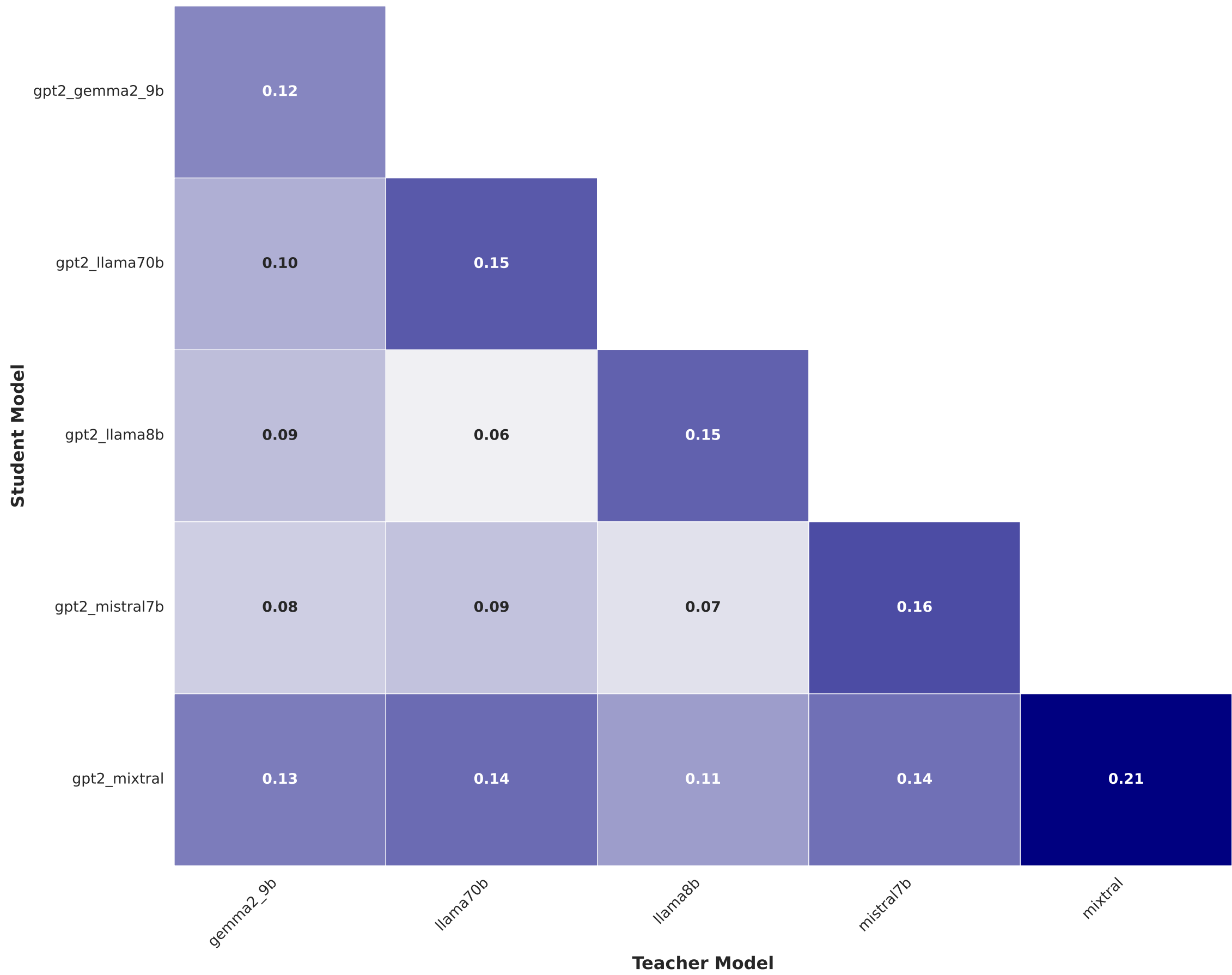
Rouge L F - Student vs Teacher Models (original_len)
