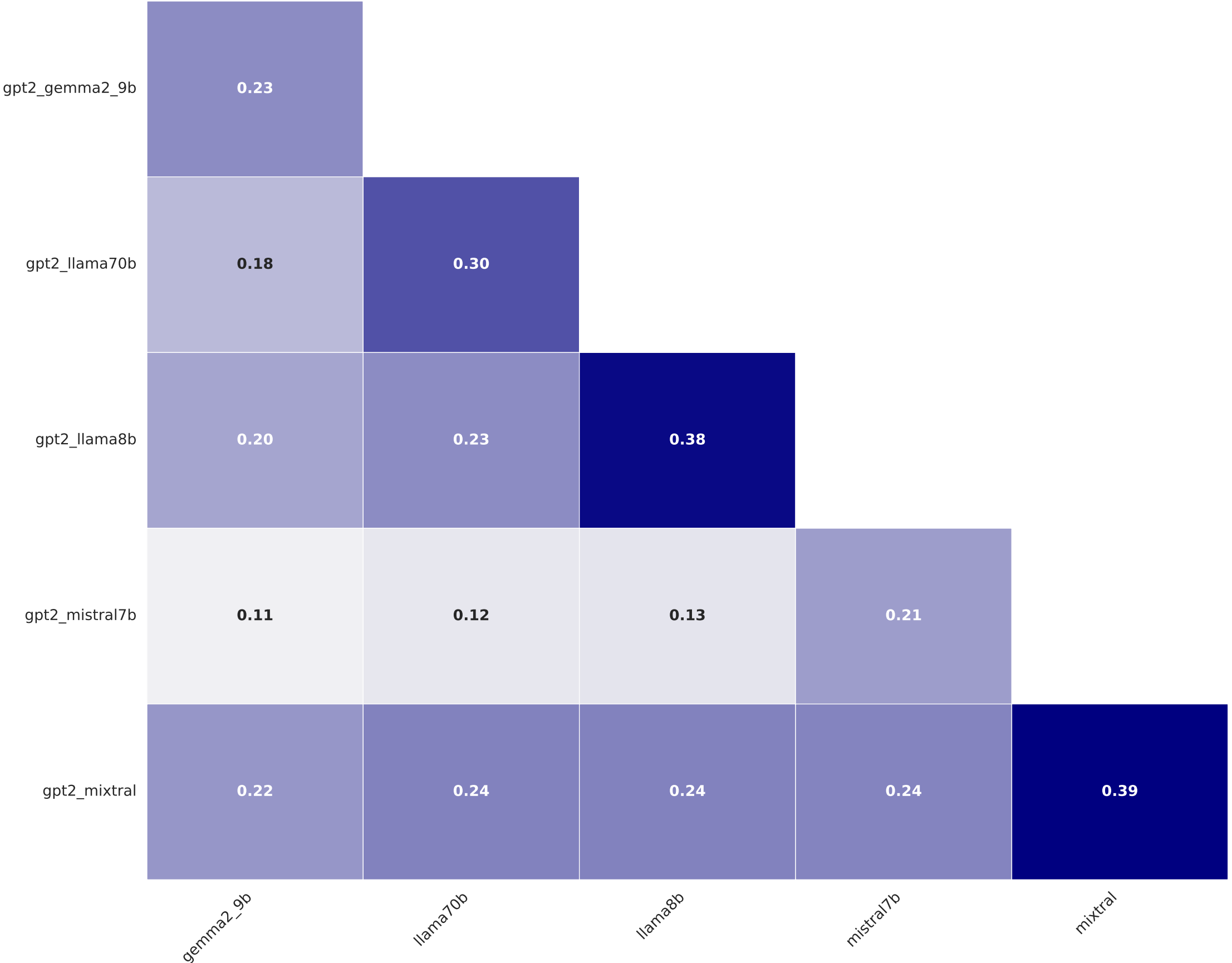
Cosine Similarity - Student vs Teacher Models (original_len)
