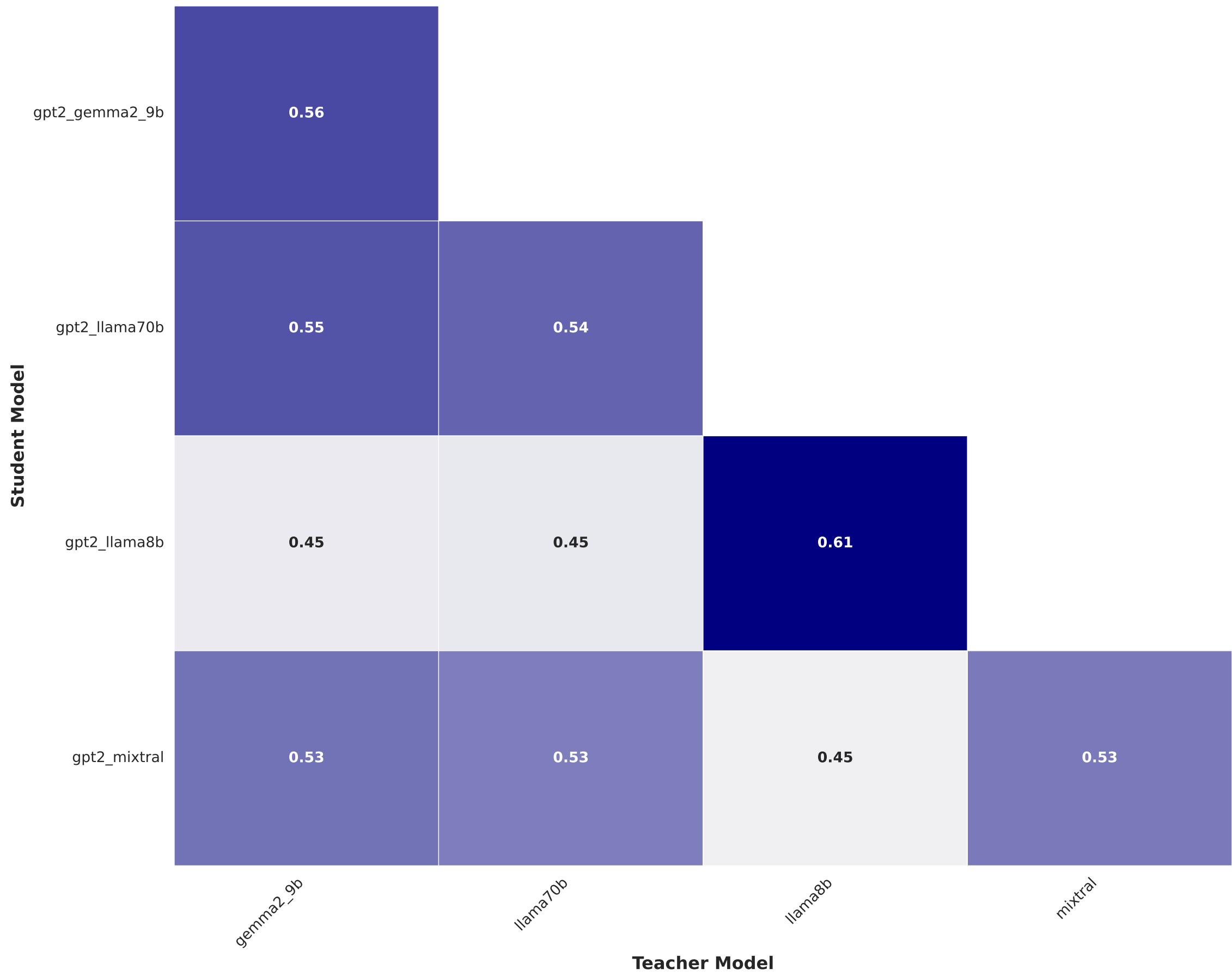
Cosine Similarity - Student vs Teacher Models (truncated)
