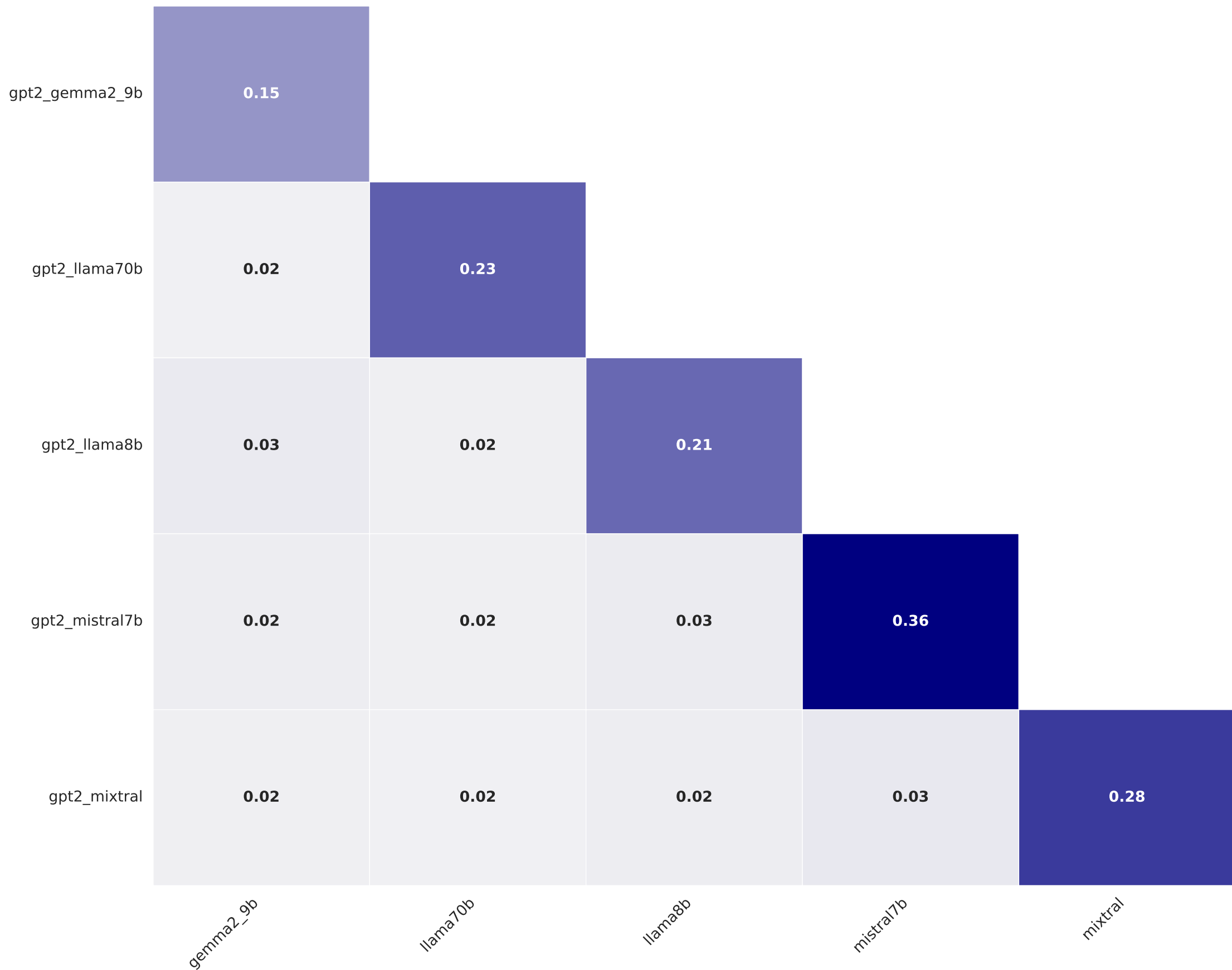
Rouge 2 F - Student vs Teacher Models (original_len)
