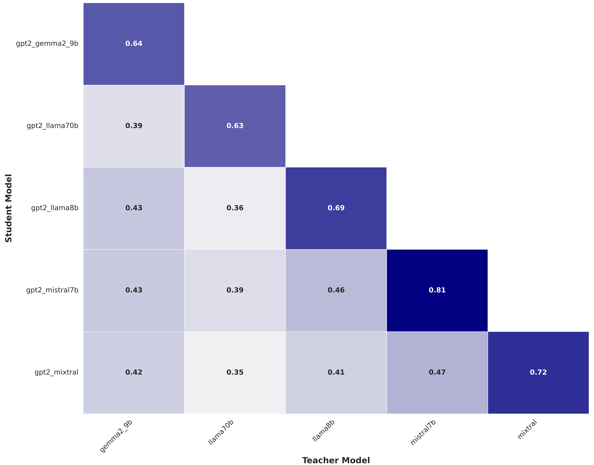
Cosine Similarity - Student vs Teacher Models (original_len)
