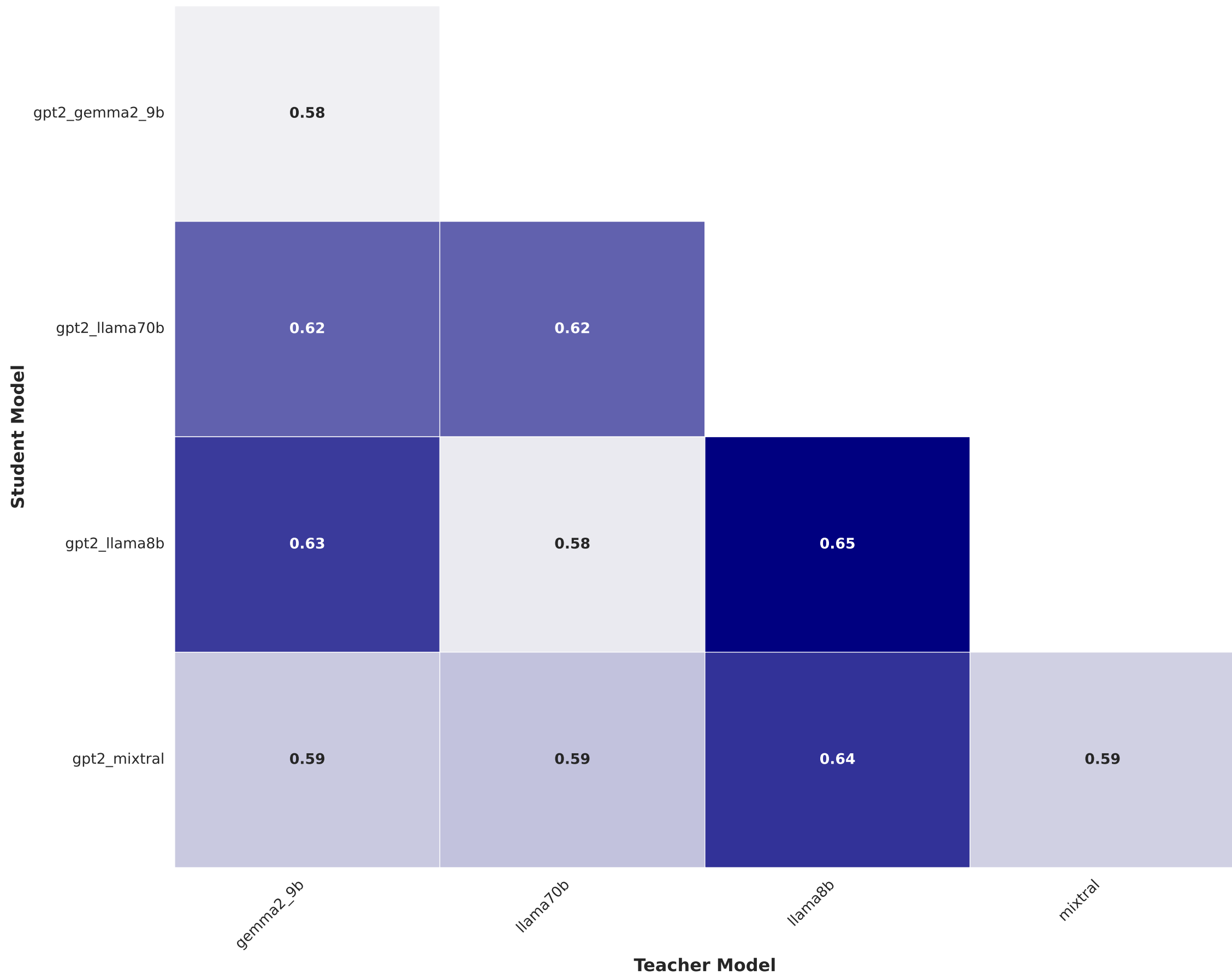
Rouge 1 F - Studentvs Teacher Models (truncated)
