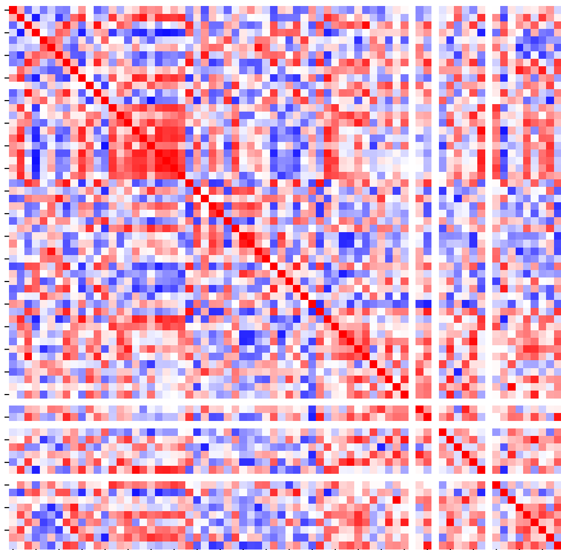
Trained
