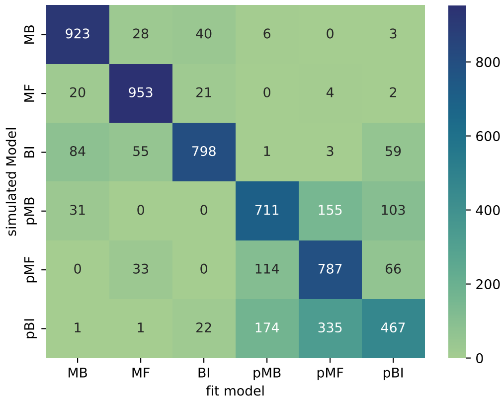
Raw Count Matrix for Current Models
