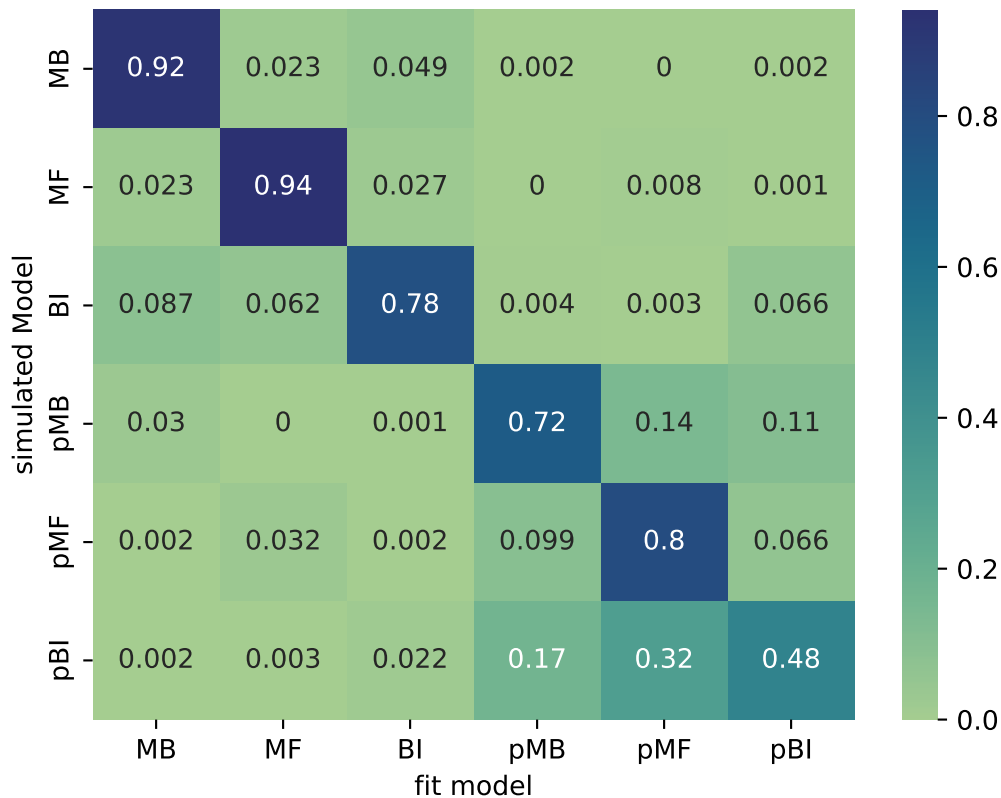
Confusion Matrix for Current Models
