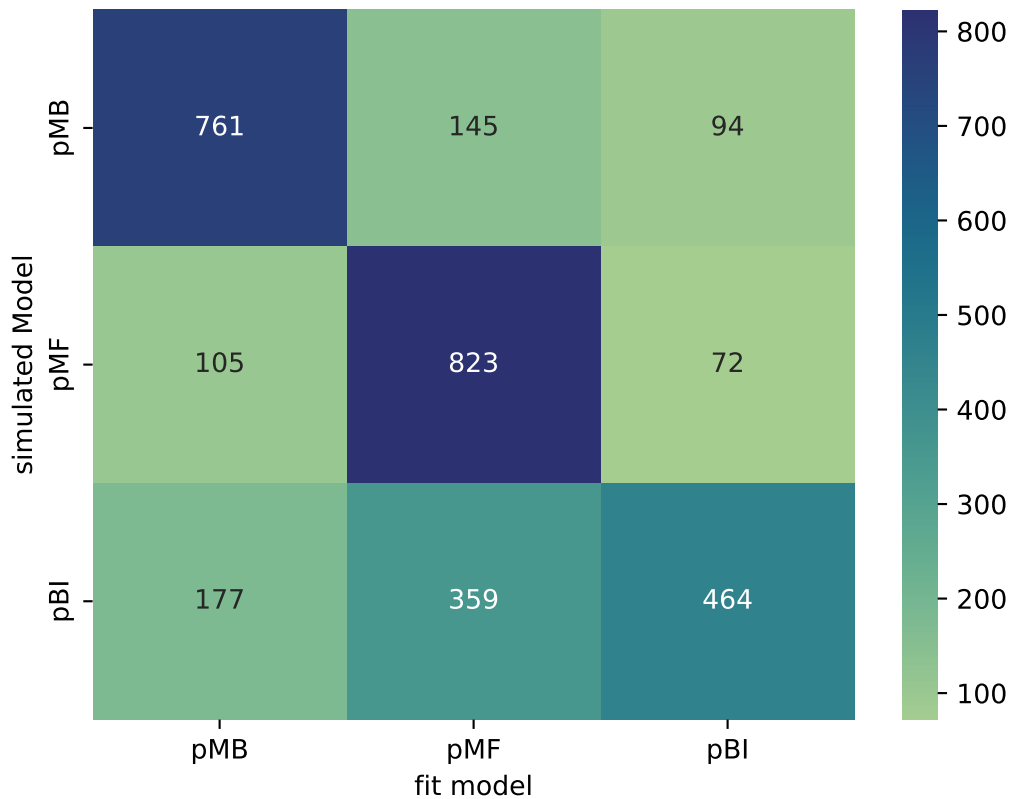
Raw Count Matrix for Models w Preservation
