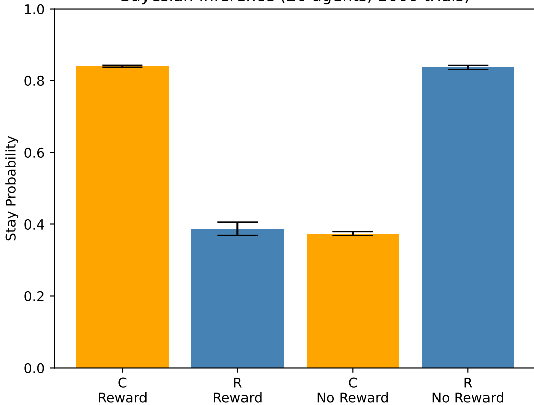
Bayesian Inference (20 agents, 1000 trials)
