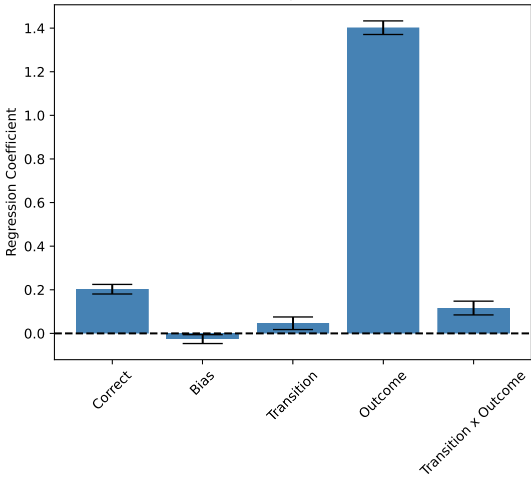
Model Free (20 agents, 1000 trials)
