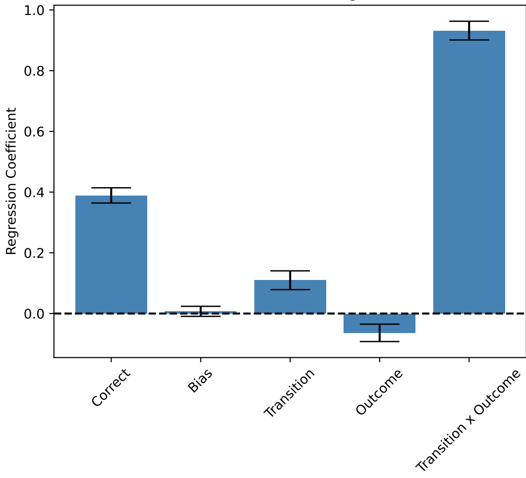
Model Based Perseveration (20 agents, 1000 trials)
