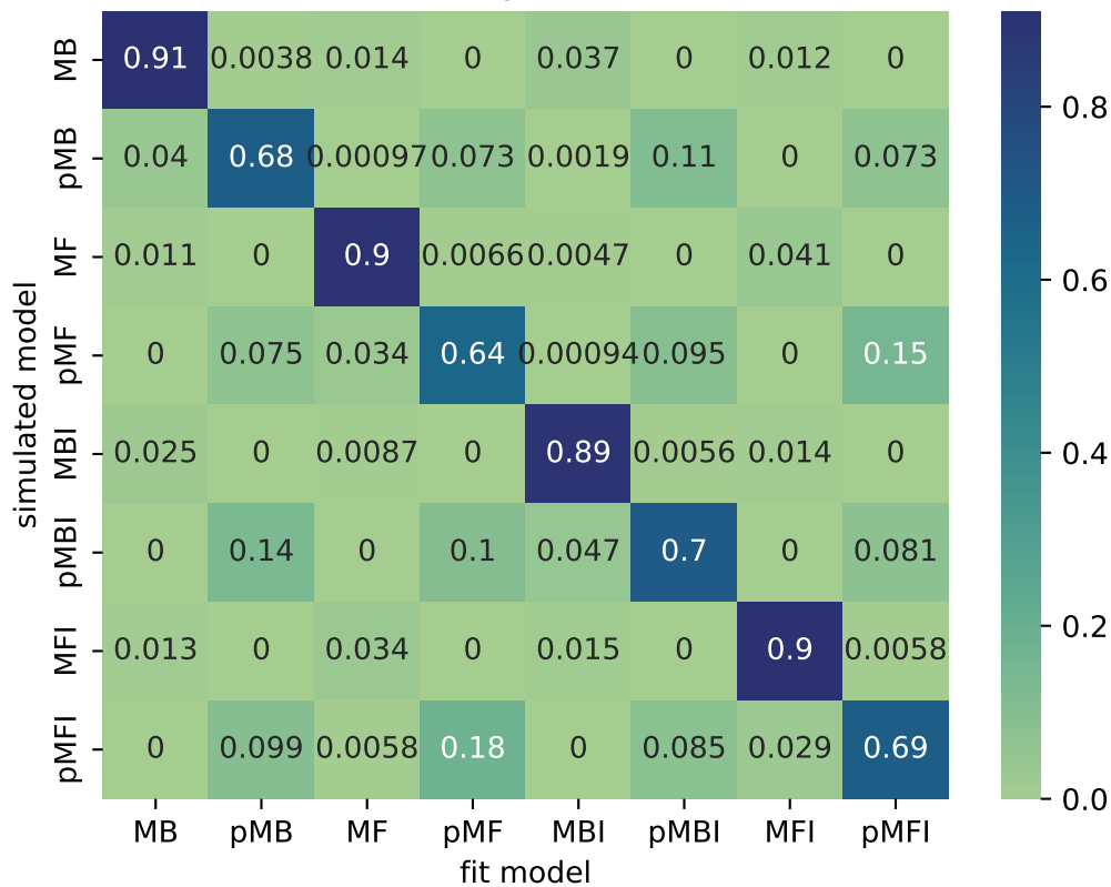
Model Rexcovery: Inverison Matrix
