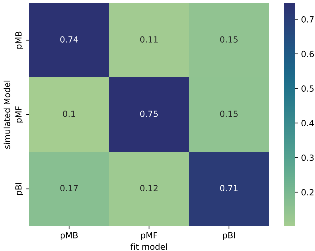
Confusion Matrix for Models w Perseveration
