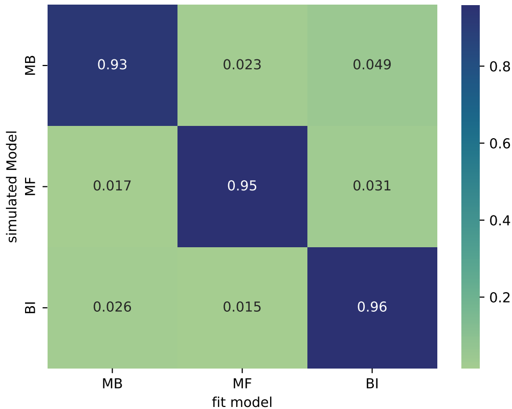
Confusion Matrix for Models w/o Perseveration
