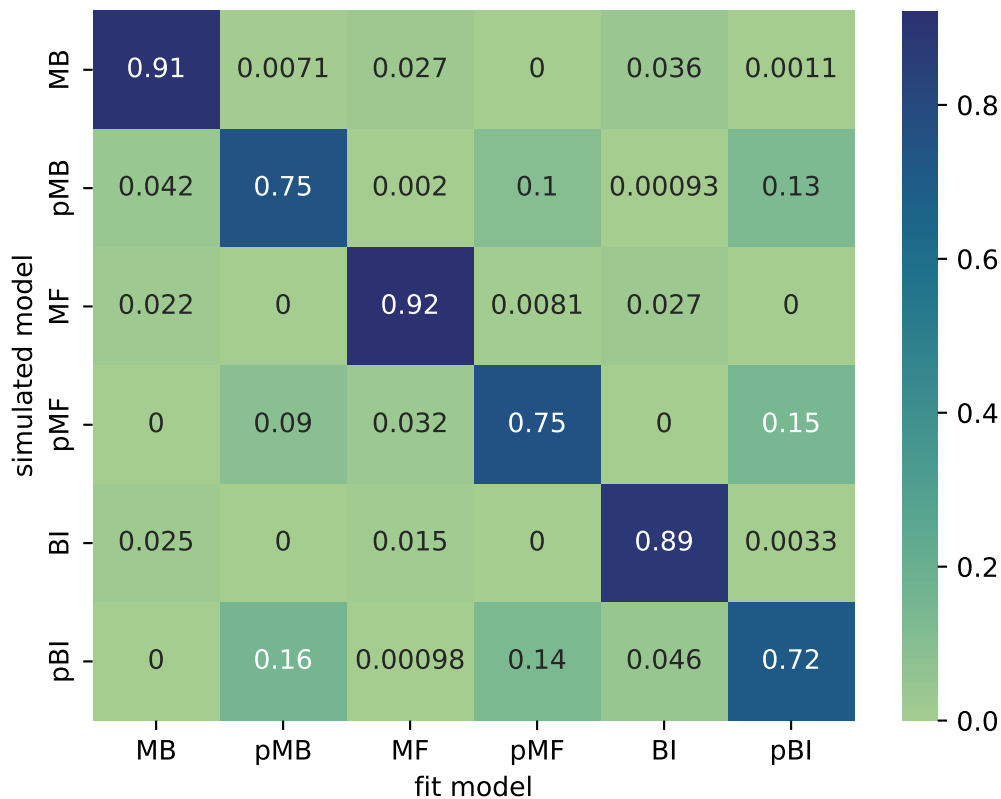
Inversion Matrix for All Current Models
