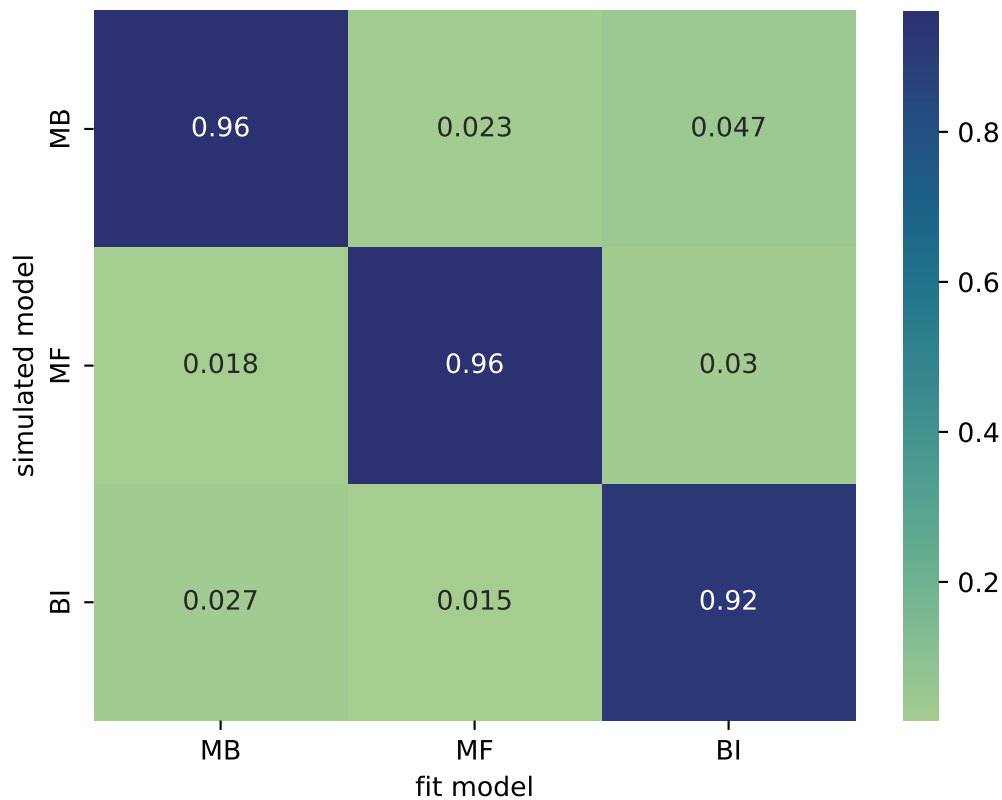
Inversion Matrix for Models w/o Perseveration
