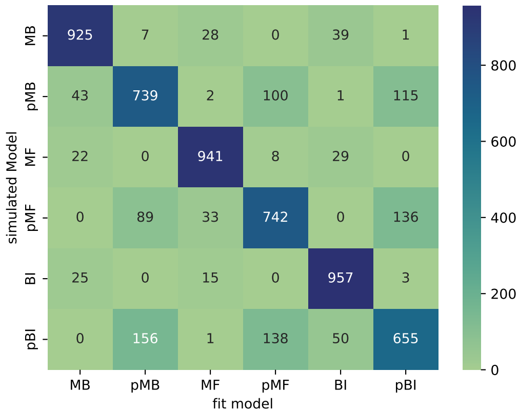
Raw Count Matrix for All Current Models
