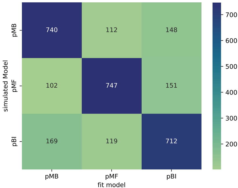
Raw Count Matrix for Models w Perseveration
