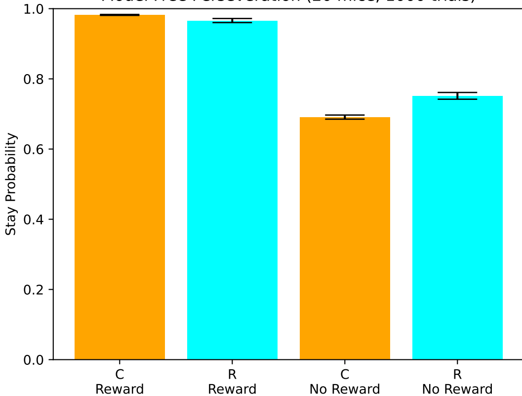
Model Free Perseveration (20 mice, 1000 trials)
