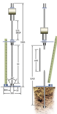
16-T0012/D Schematic operating principle
