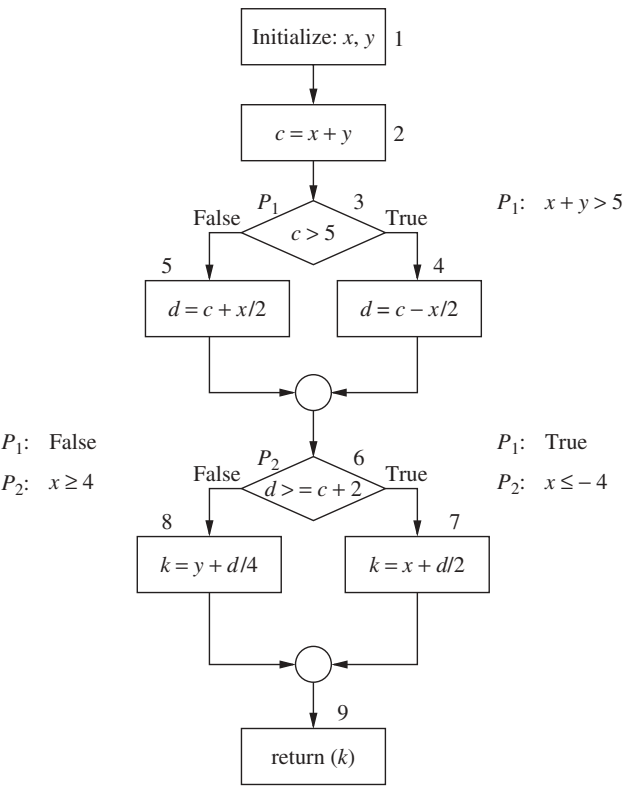
Figure 6.3 Control flow graph representation of the function in Figure 6.2.
