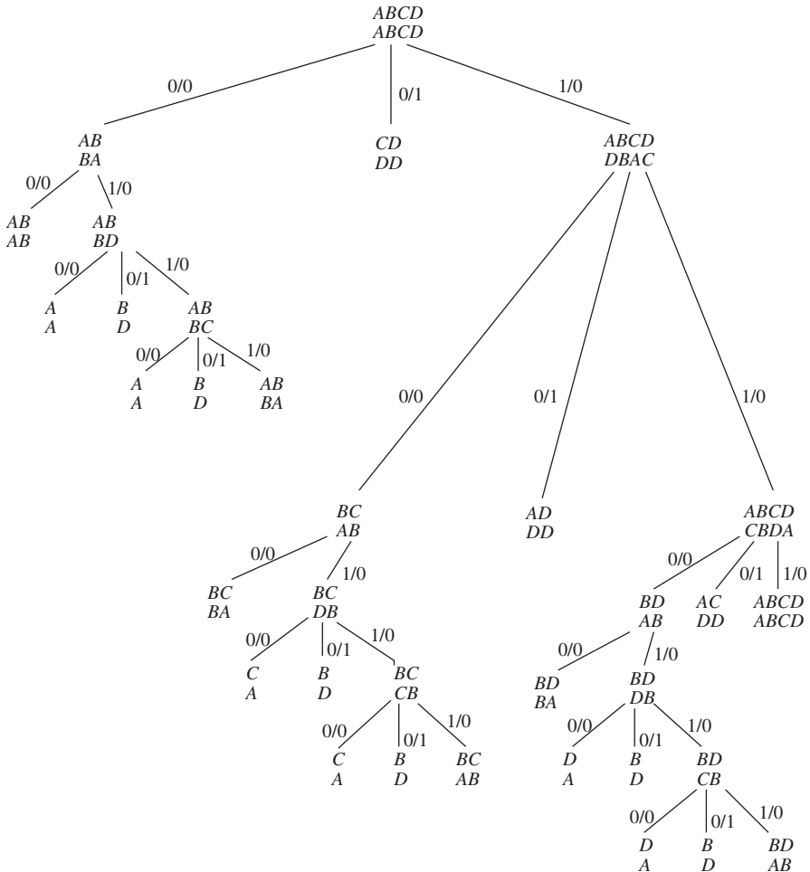
Figure 10.13 UIO tree for G_1 in Figure 10.12. (From ref. 5. © 1997 IEEE.)
