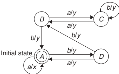
Figure 10.17 FSM that does not possess distinguishing sequence. (From ref. 11. © 1994 IEEE.)
