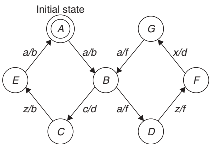
Figure 10.50 FSM H.
