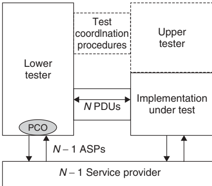
Figure 10.25 Remote architecture.
