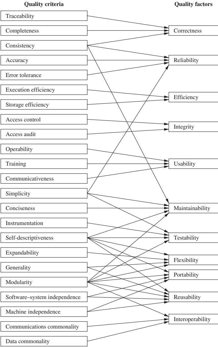
Figure 17.1 Relation between quality factors and quality criteria [6].
