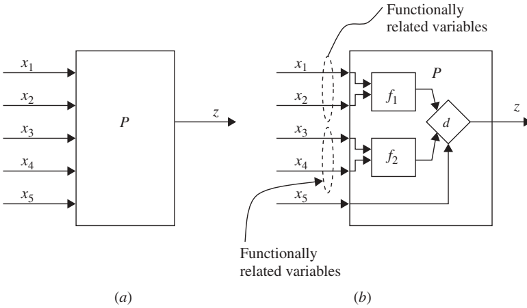
Figure 9.3 Functionally related variables.
