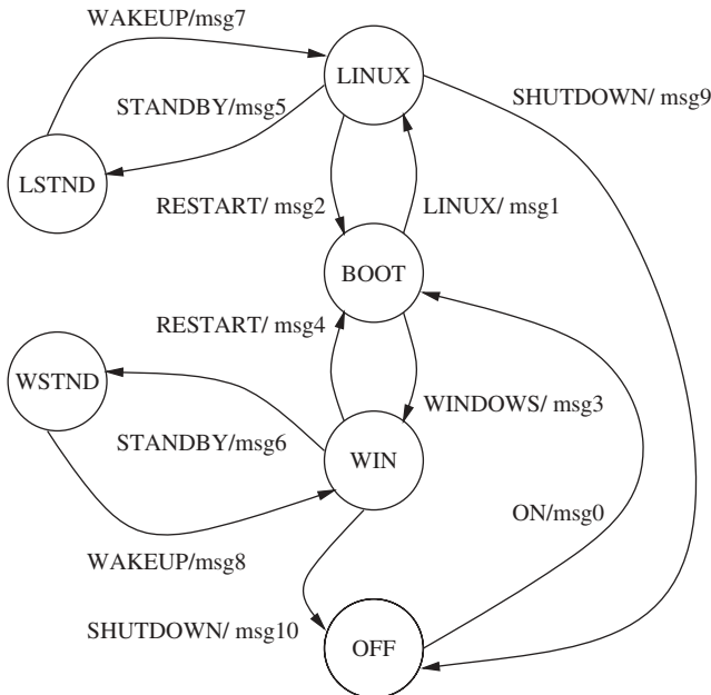
Figure 10.4 FSM model of a dual-boot laptop computer.
