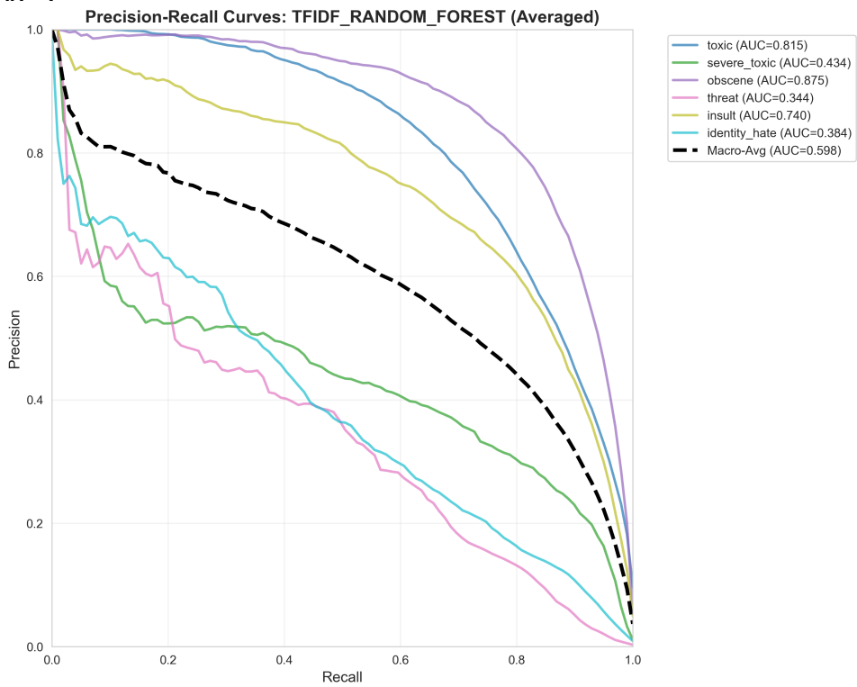
Pr Curves
