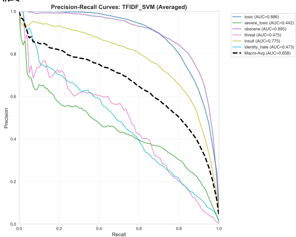
Pr Curves
