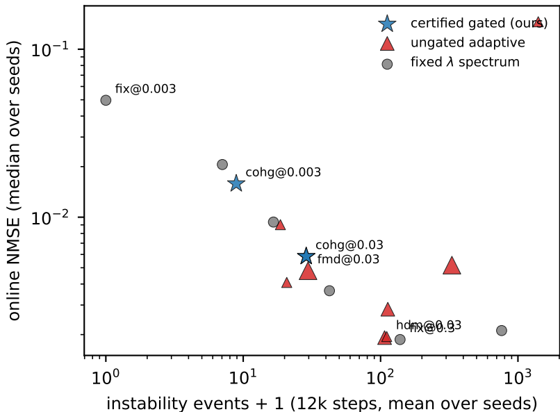
Safety-performance Pareto on drifting streams (marker size \propto HVPs/step: cost-normalized view)
