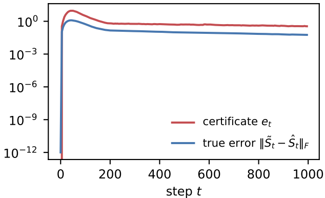
(a) anytime certificate vs. true error (teacher-student, \gamma=0.9 , r=4 , K=5 )
