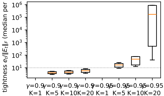
(b) tightness across discount & laziness (10 seeds; \gamma = 0.95 , K \geq 10 crosses \gamma\bar{\rho} = 1 )
