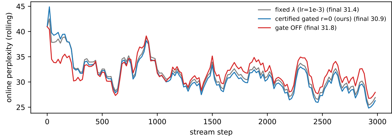
GPT-2 124M streaming TTA under domain shift (wiki → news → code)
