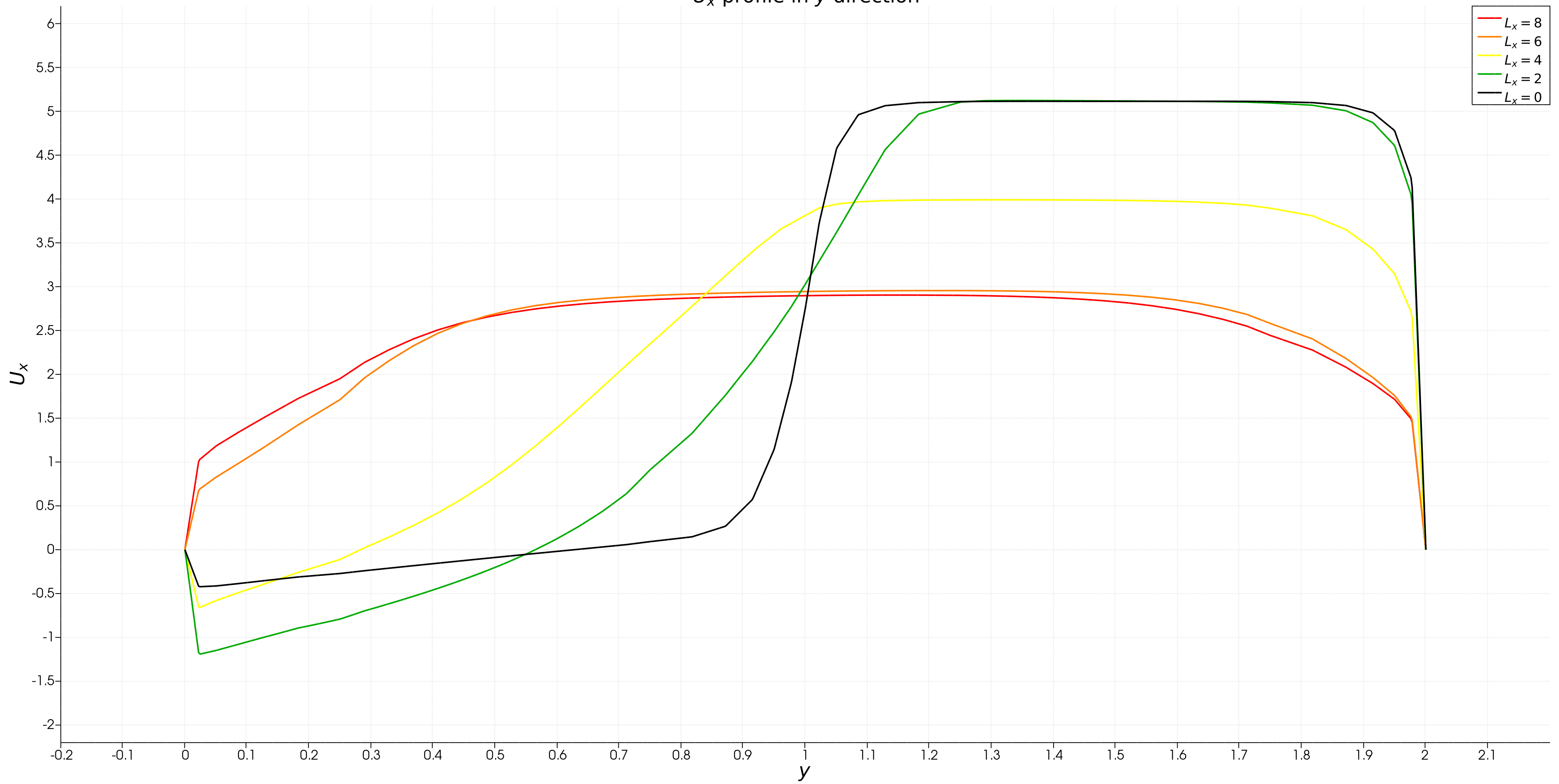
U_x profile in y direction
