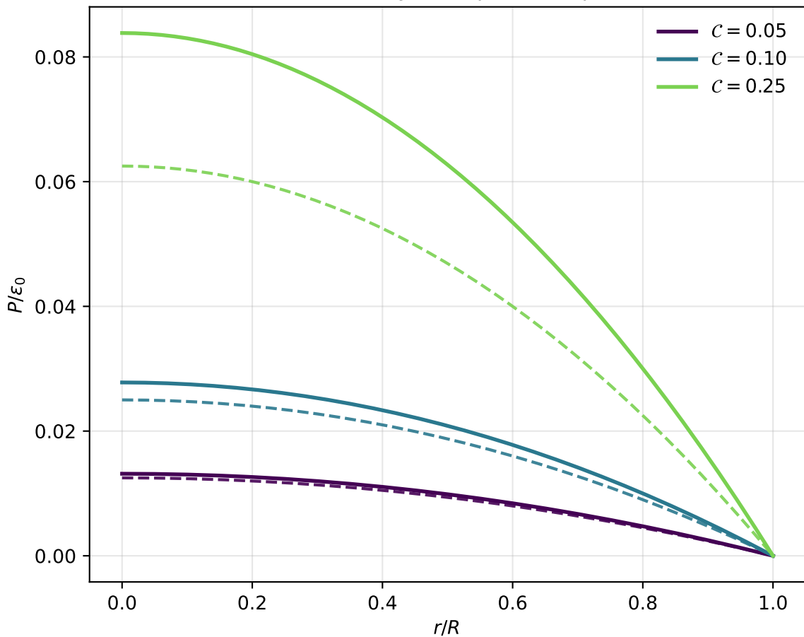
Uniform-density star: pressure profiles
