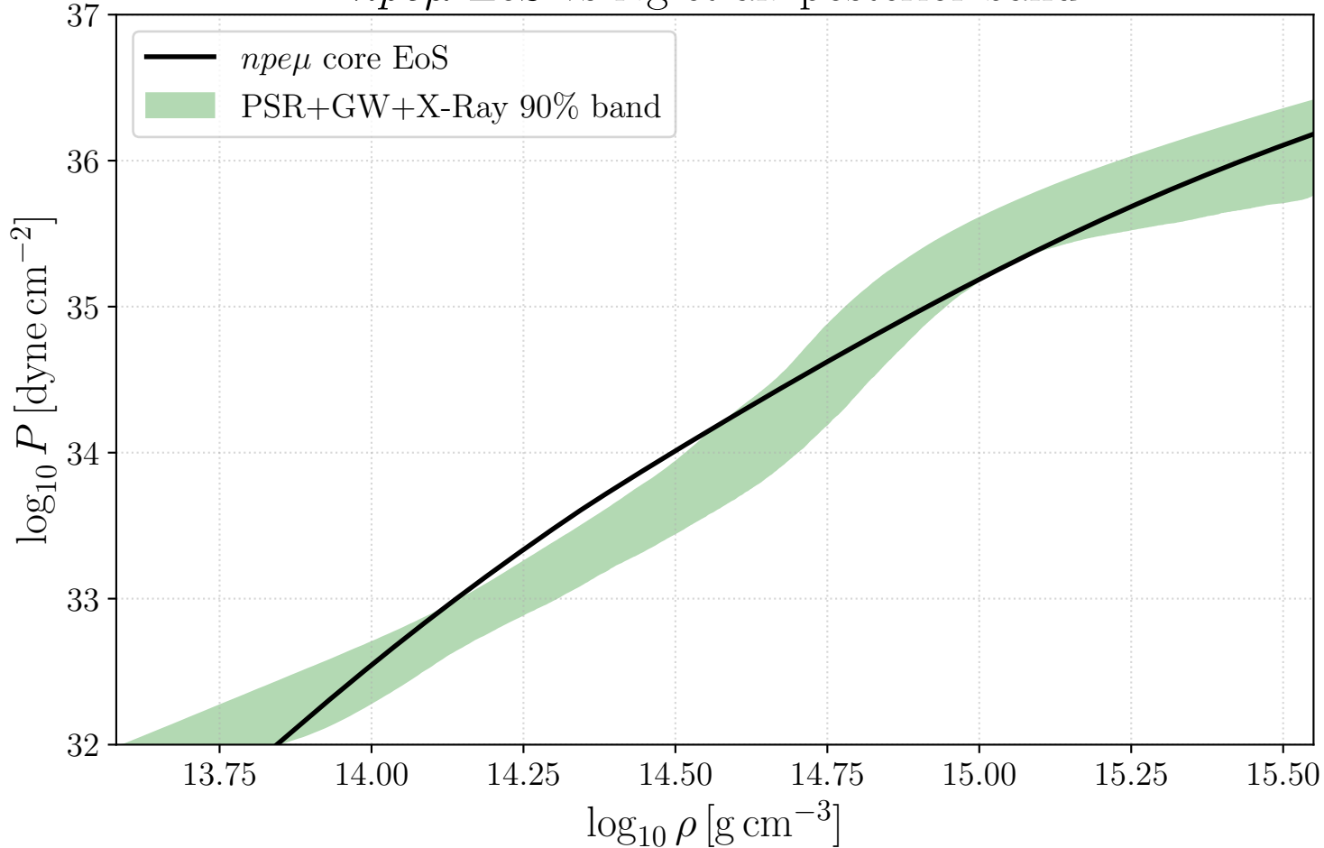
npe\mu EoS vs Ng et al. posterior band
