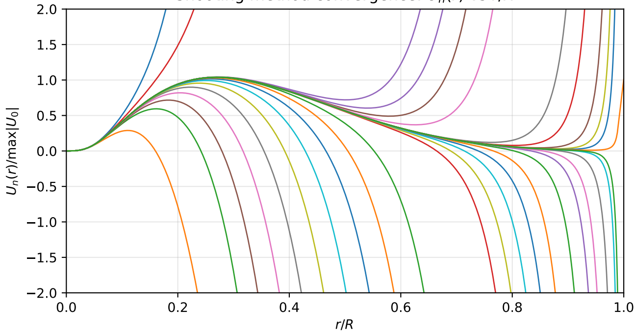
Shooting method convergence: U_n(r) vs r/R
