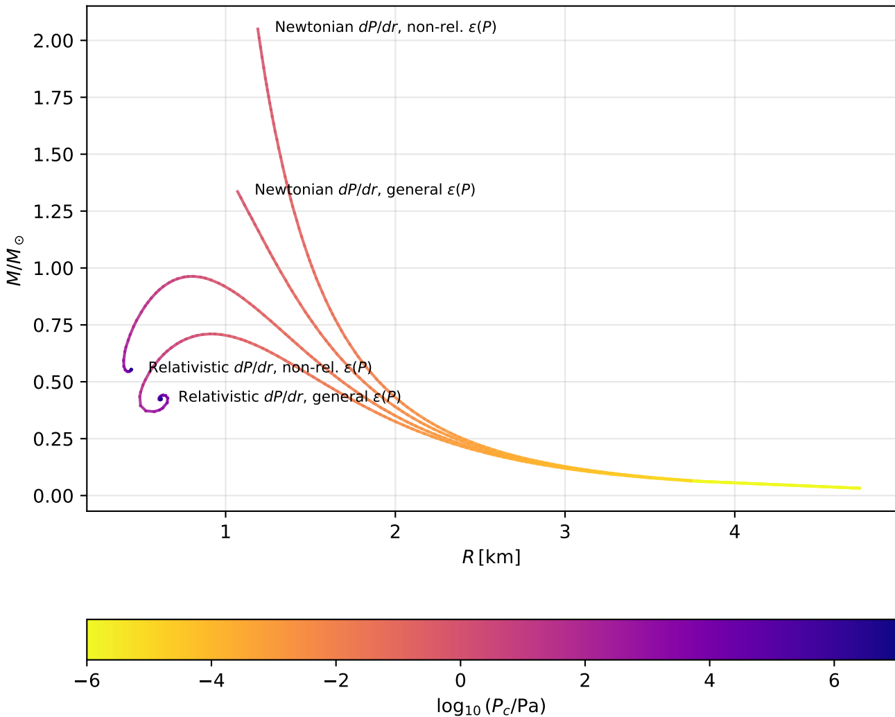
Mass-radius diagram for ideal neutron stars
