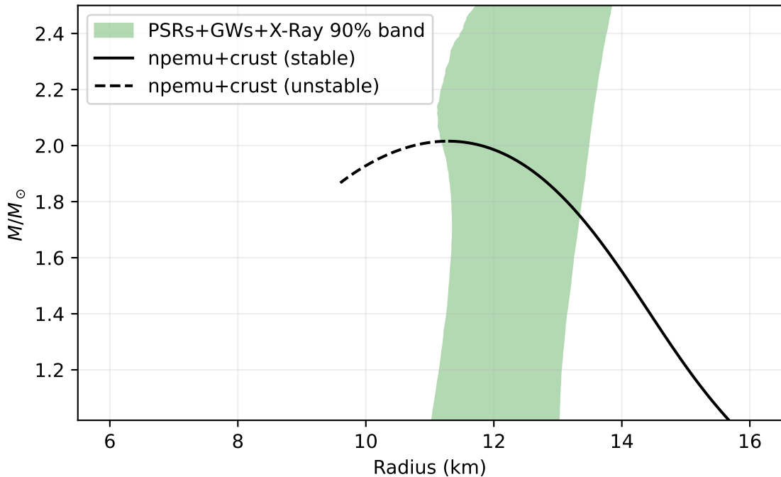
Mass-Radius Relation vs Ng et al. posterior band
