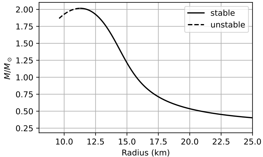
Mass-Radius Relation
