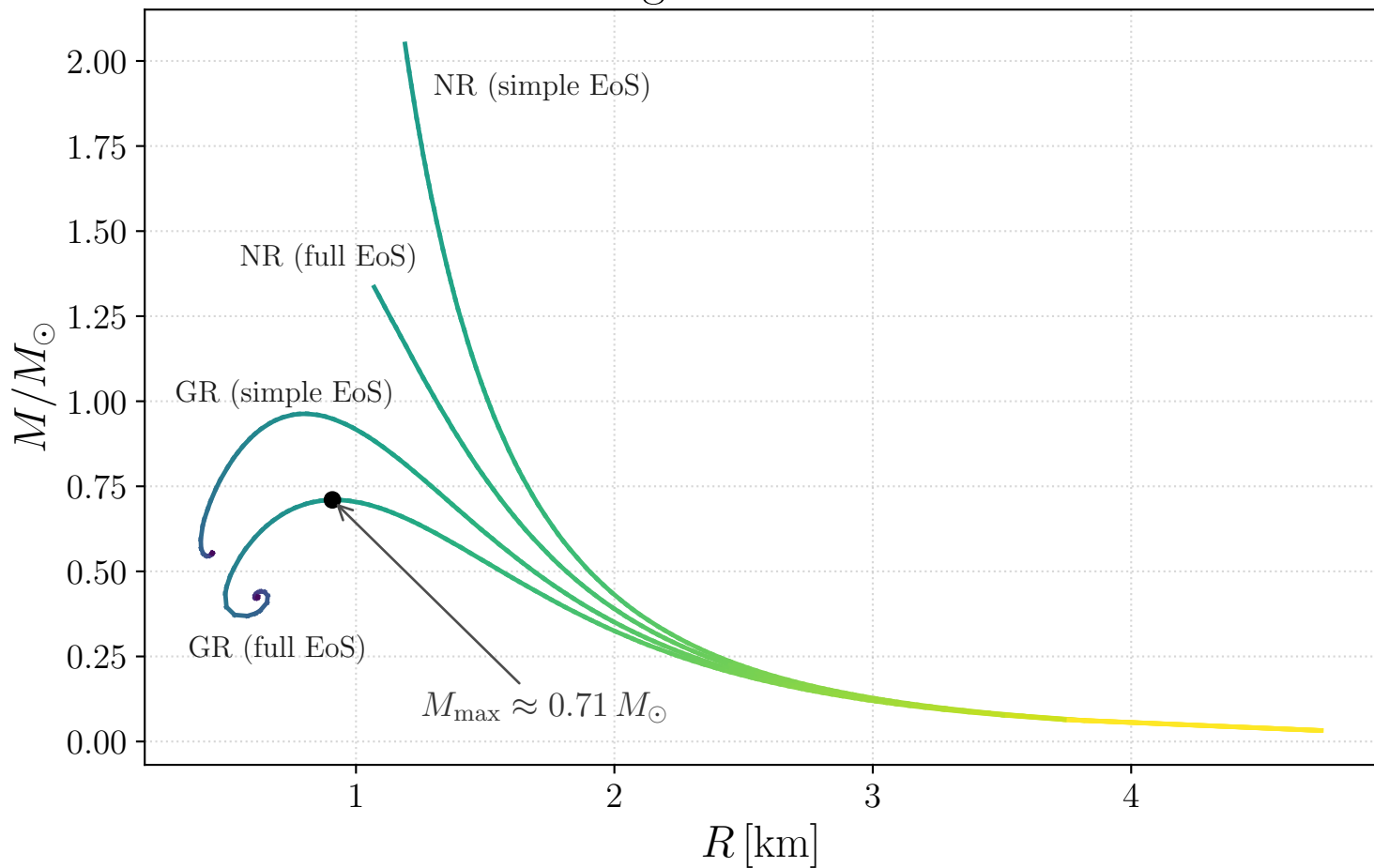
Mass-radius diagram for ideal neutron stars
