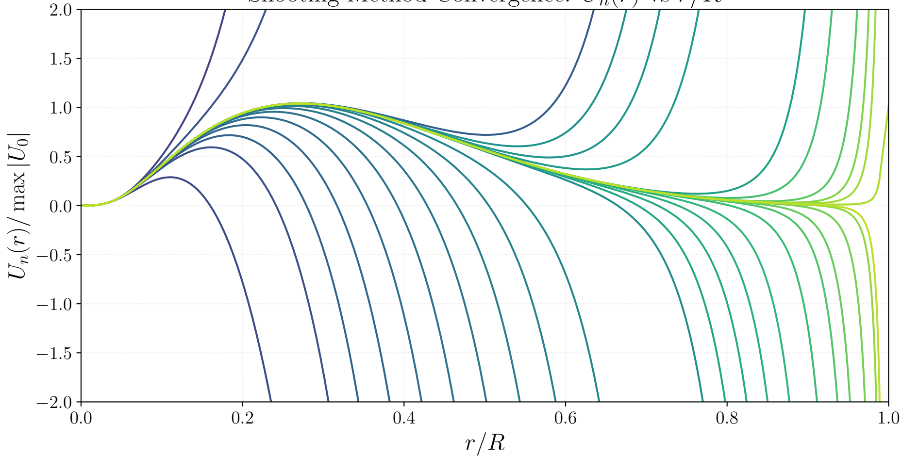
Shooting Method Convergence: U_n(r) vs r/R
