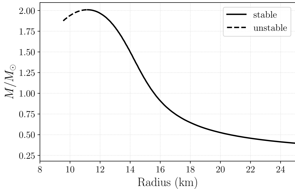
Mass–Radius Relation
