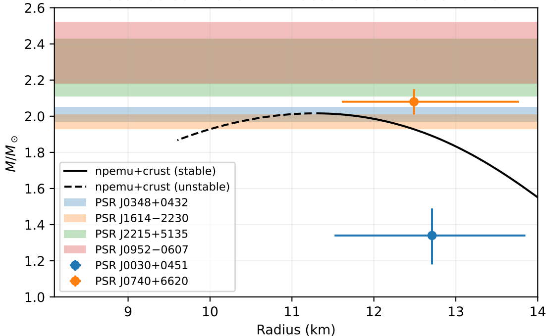
Mass-radius relation with observational constraints
