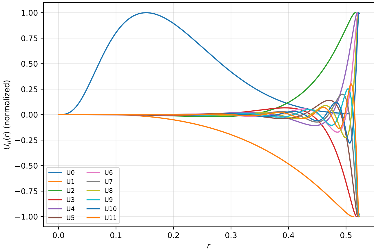
Normalized radial eigenfunctions
