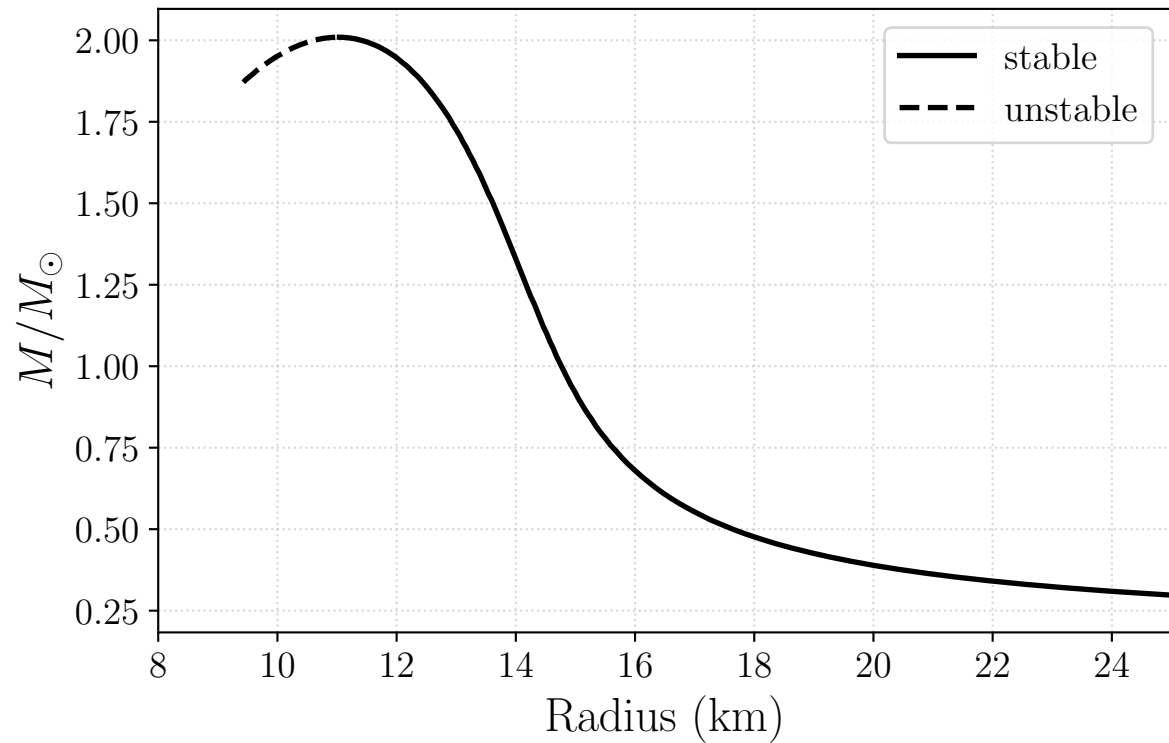
Mass–Radius Relation
