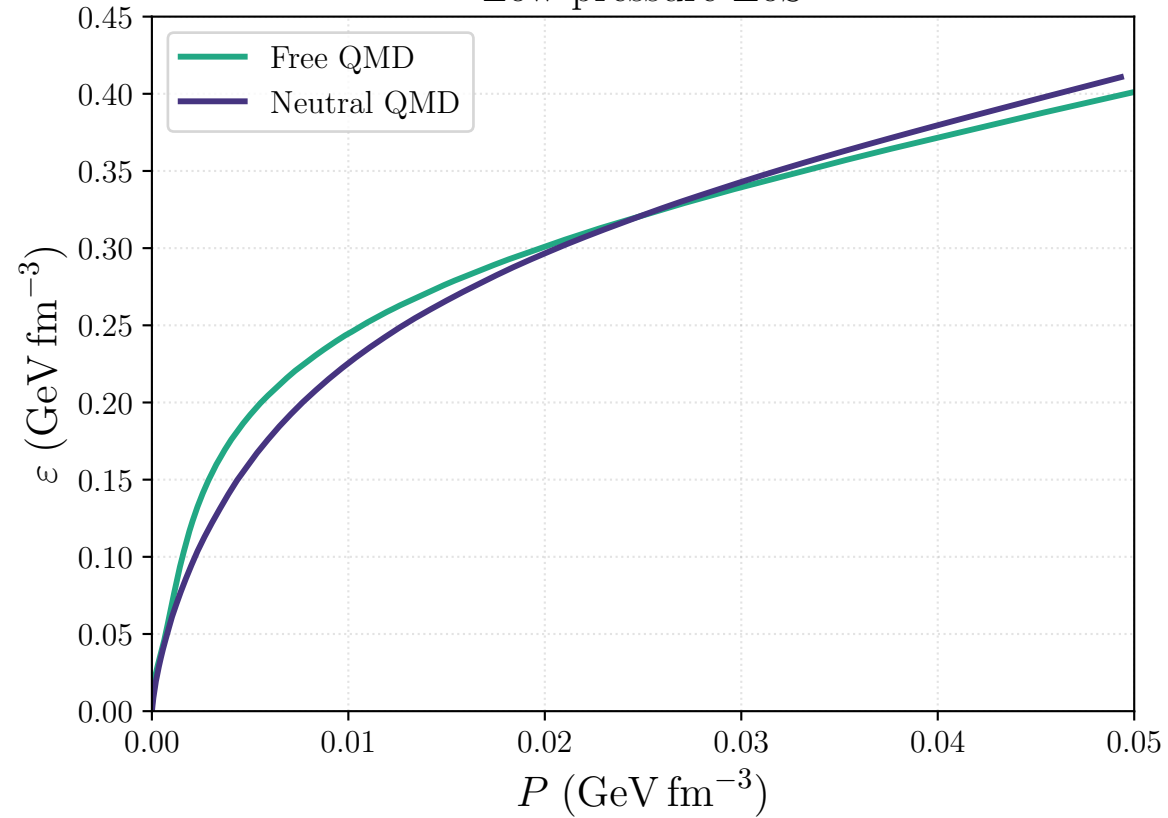
Low-pressure EoS
