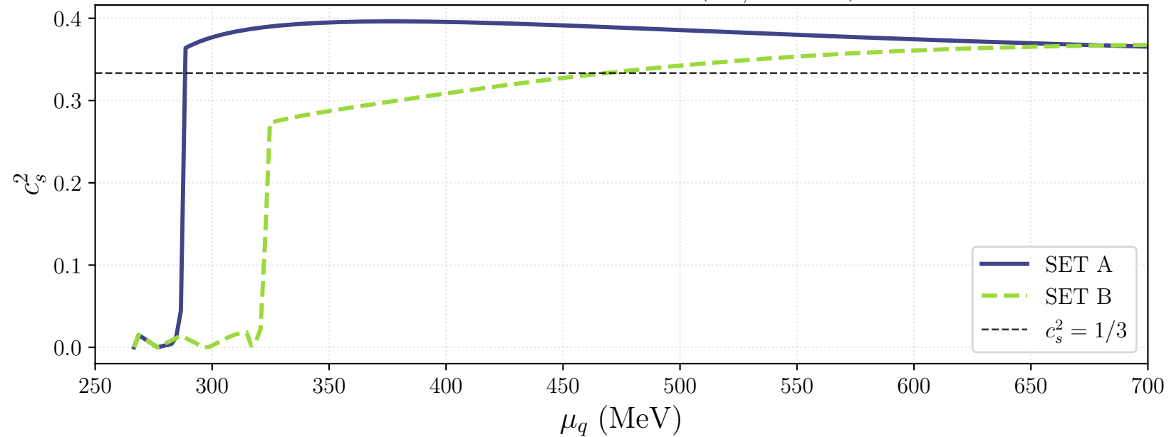
Speed of sound squared ( \Omega_{1,\text{num}} = 0 )
