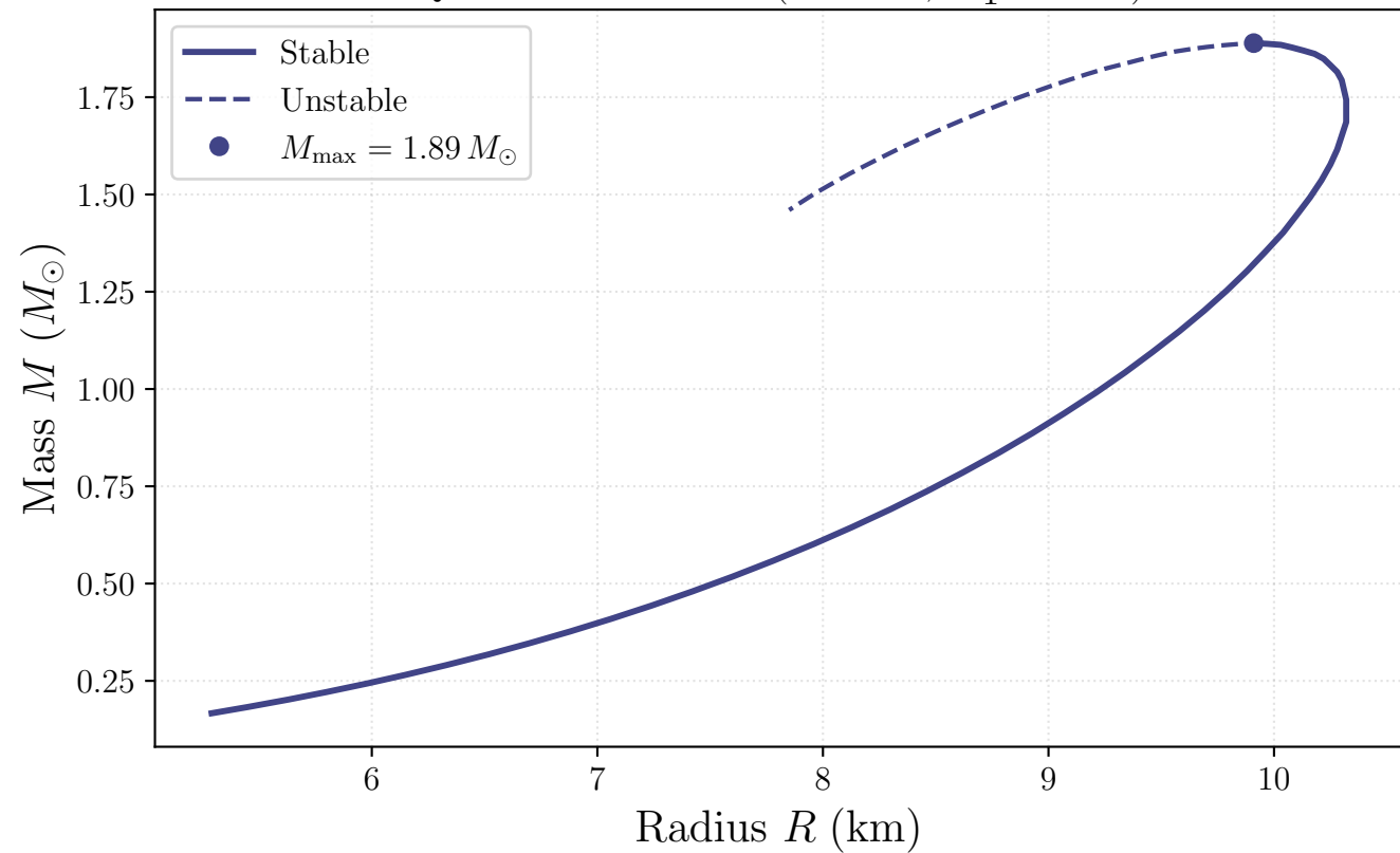
QMD mass-radius (SET_A, \Omega_1^{\text{num}} = 0 )
