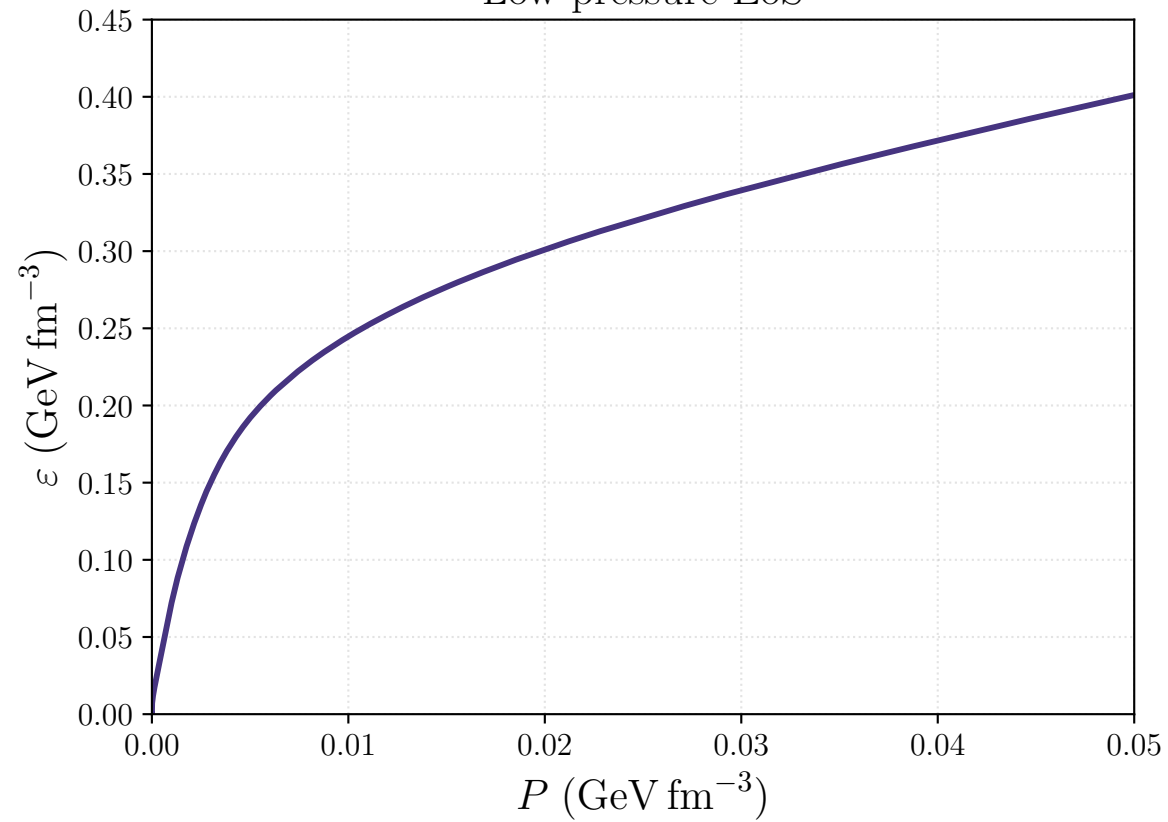
Low-pressure EoS
