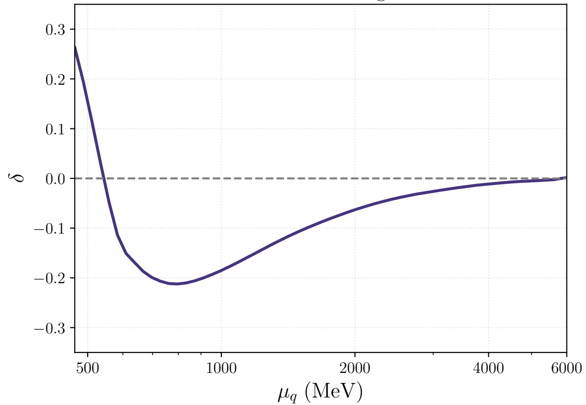
Conformal convergence
