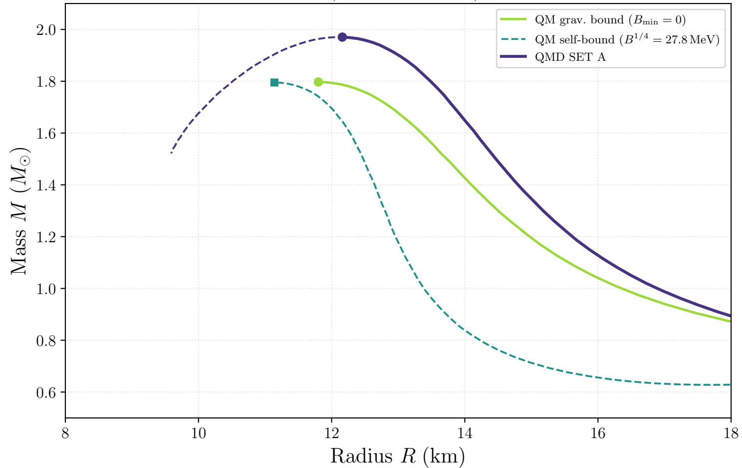
QMD vs QM ( m_\sigma = 600 MeV) mass-radius
