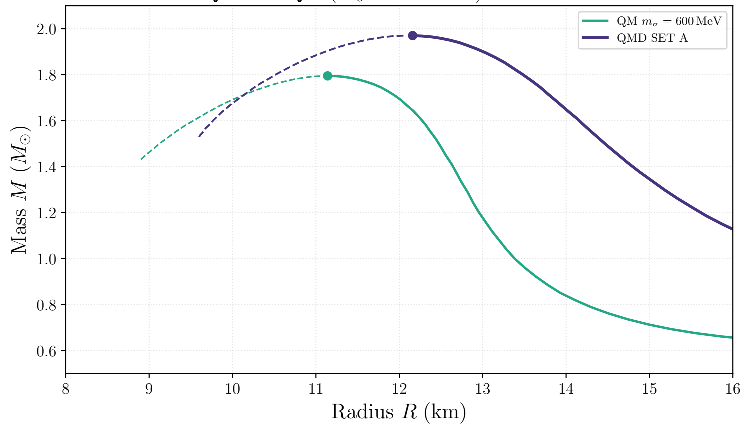
QMD vs QM ( m_\sigma = 600 MeV) mass-radius
