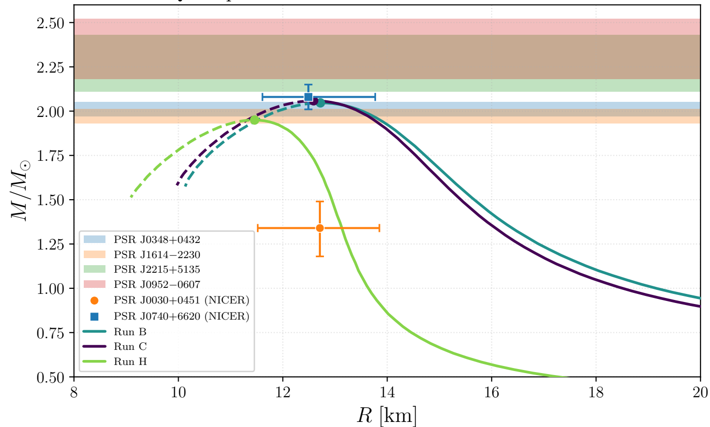
Selected QMD parameter variations and observational constraints
