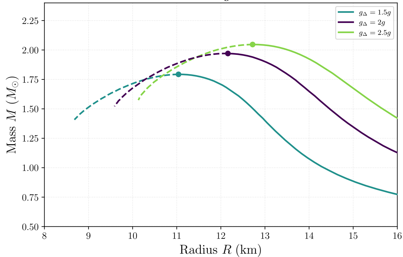
Mass-radius: g_\Delta variation
