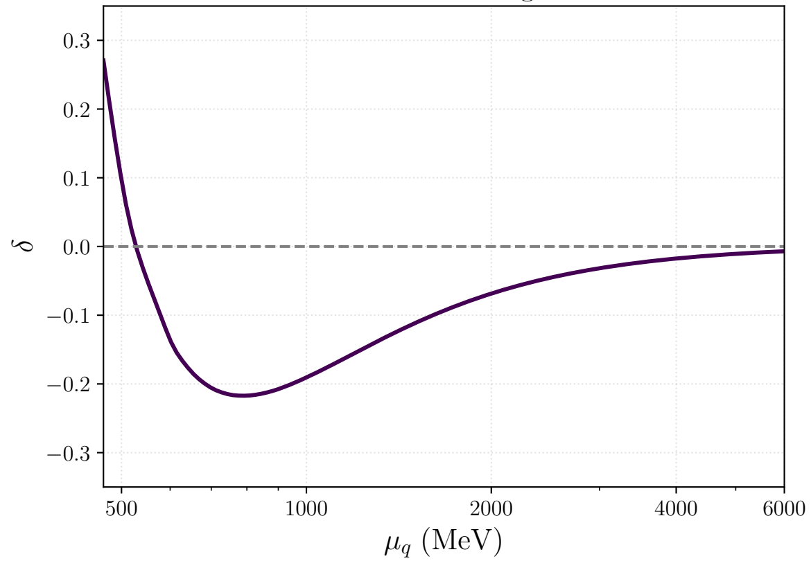
Conformal convergence
