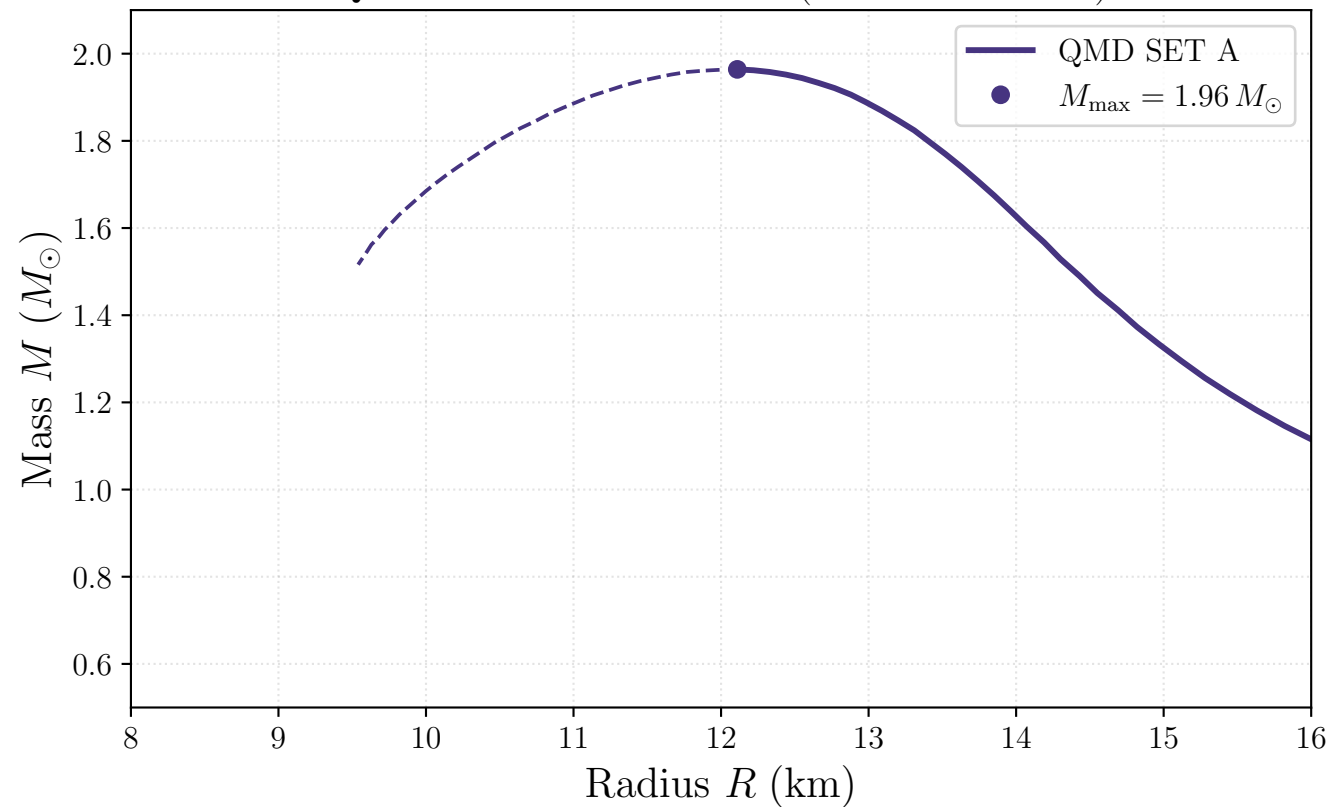
QMD stellar mass-radius (SET A baseline)
