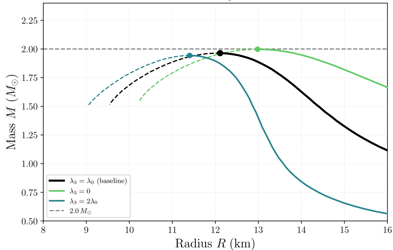
Mass-radius: \lambda_3 variation
