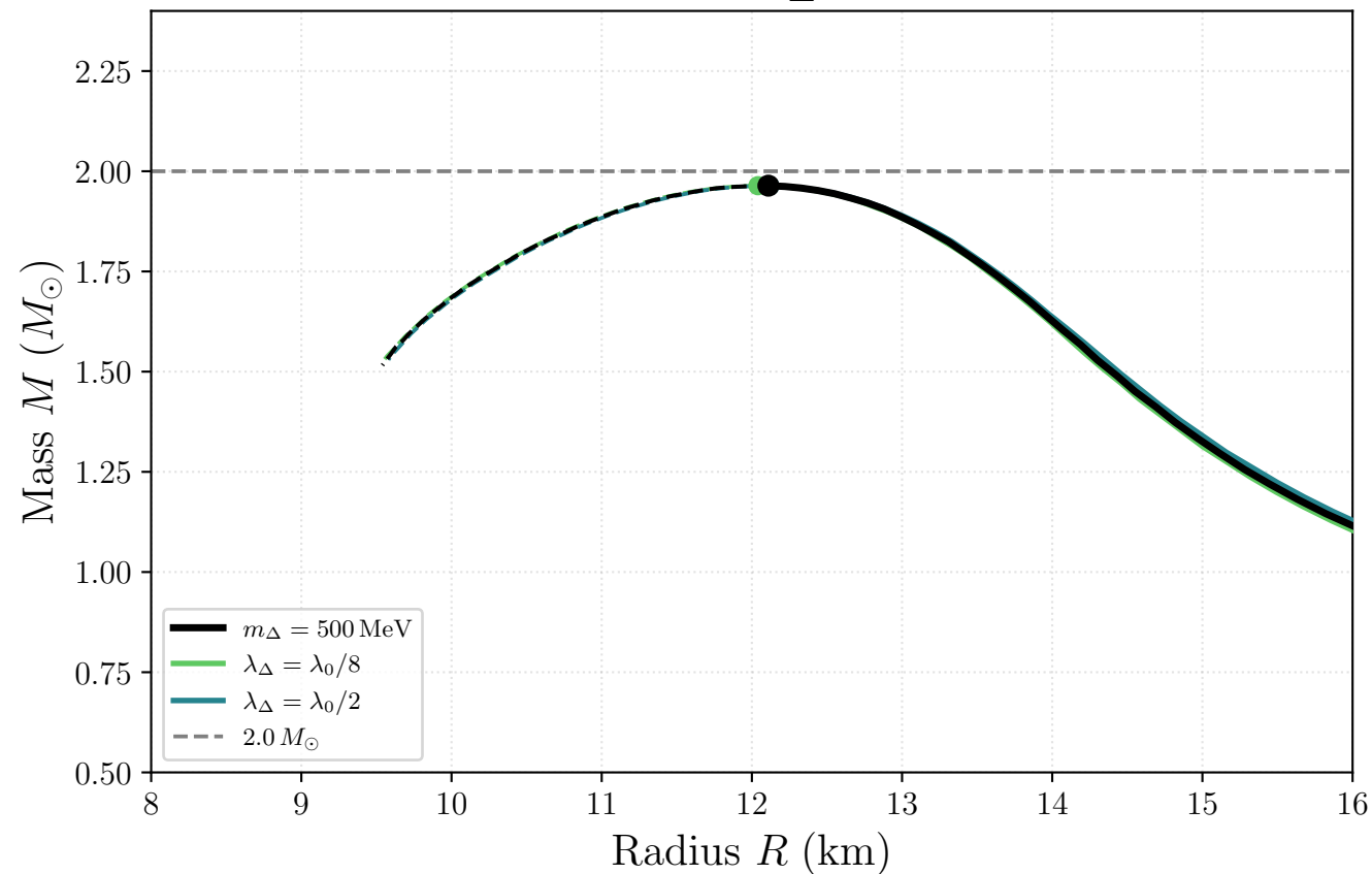
Mass-radius: \lambda_\Delta variation
