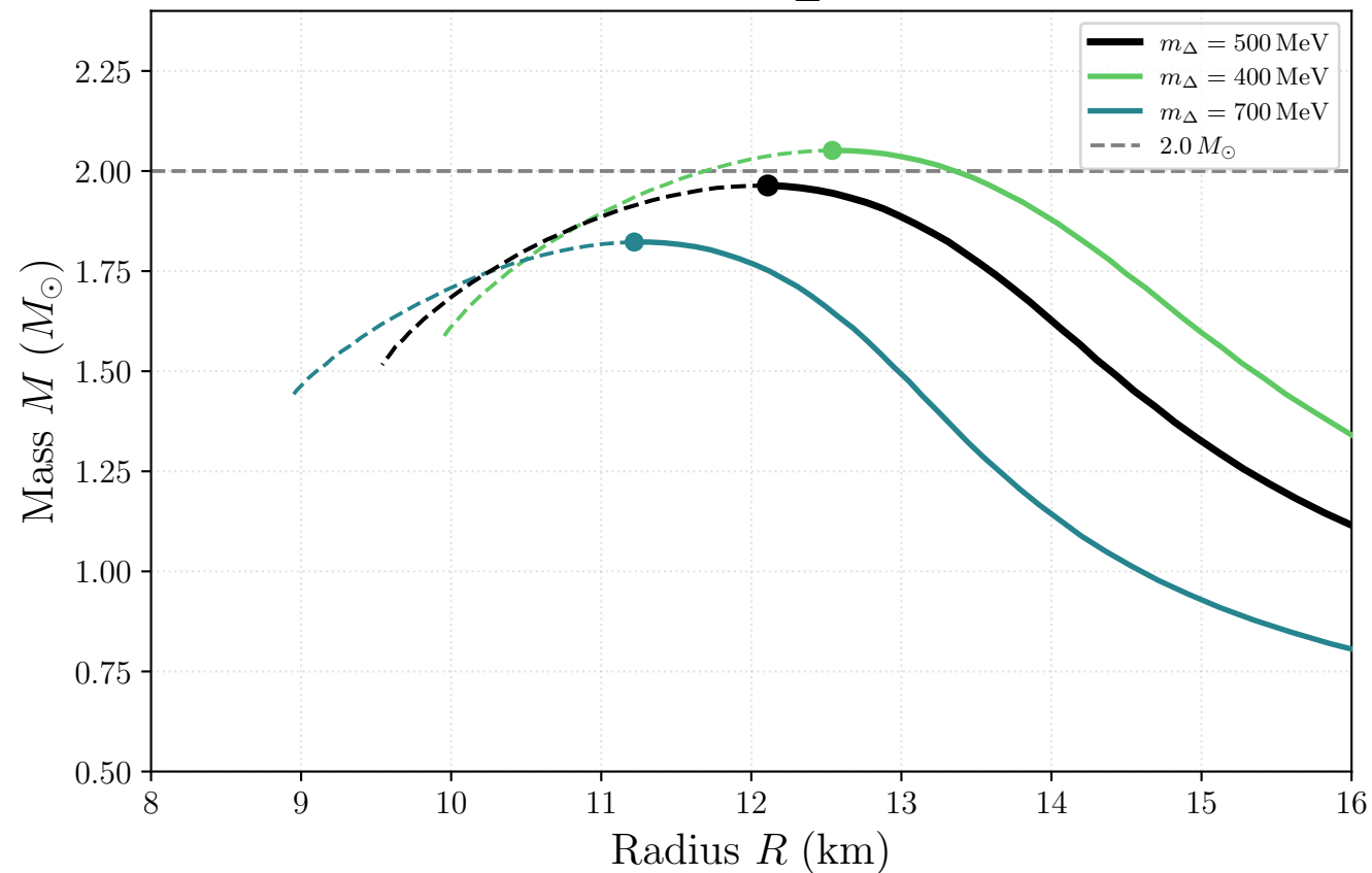
Mass-radius: m_\Delta variation
