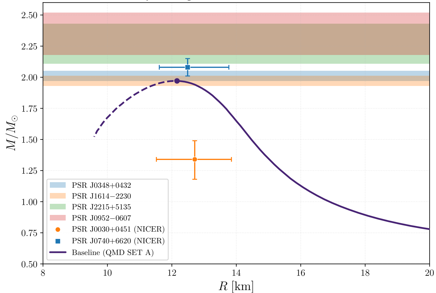
Baseline QMD sequence and observational constraints
