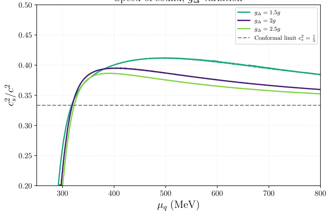
Speed of sound, g_\Delta variation
