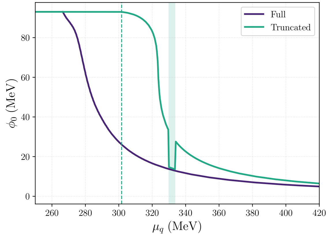
Chiral condensate
